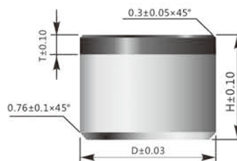
Dimensions and Tolerance
