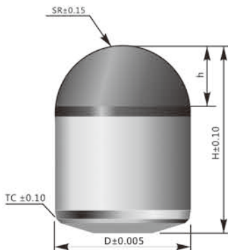
Dimensions and Tolerance
